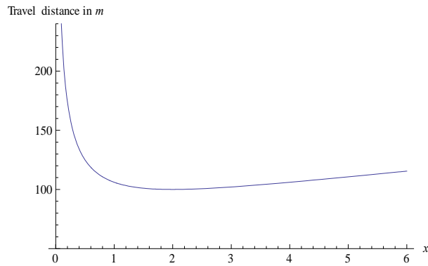
Figure 4. Travel distance \sqrt{\frac{C}{x}} + \frac{1}{2}\sqrt{Cx} as function of the warehouse length/width ratio x , for a warehouse of C=5000m^2 .
