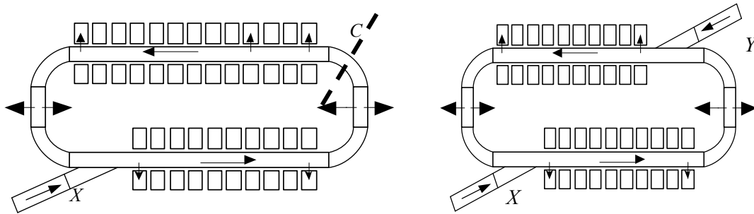
Figure 7. Loop sorter sorting to two sides with one (left) and two inducts (right). Source: Vanderlande.
